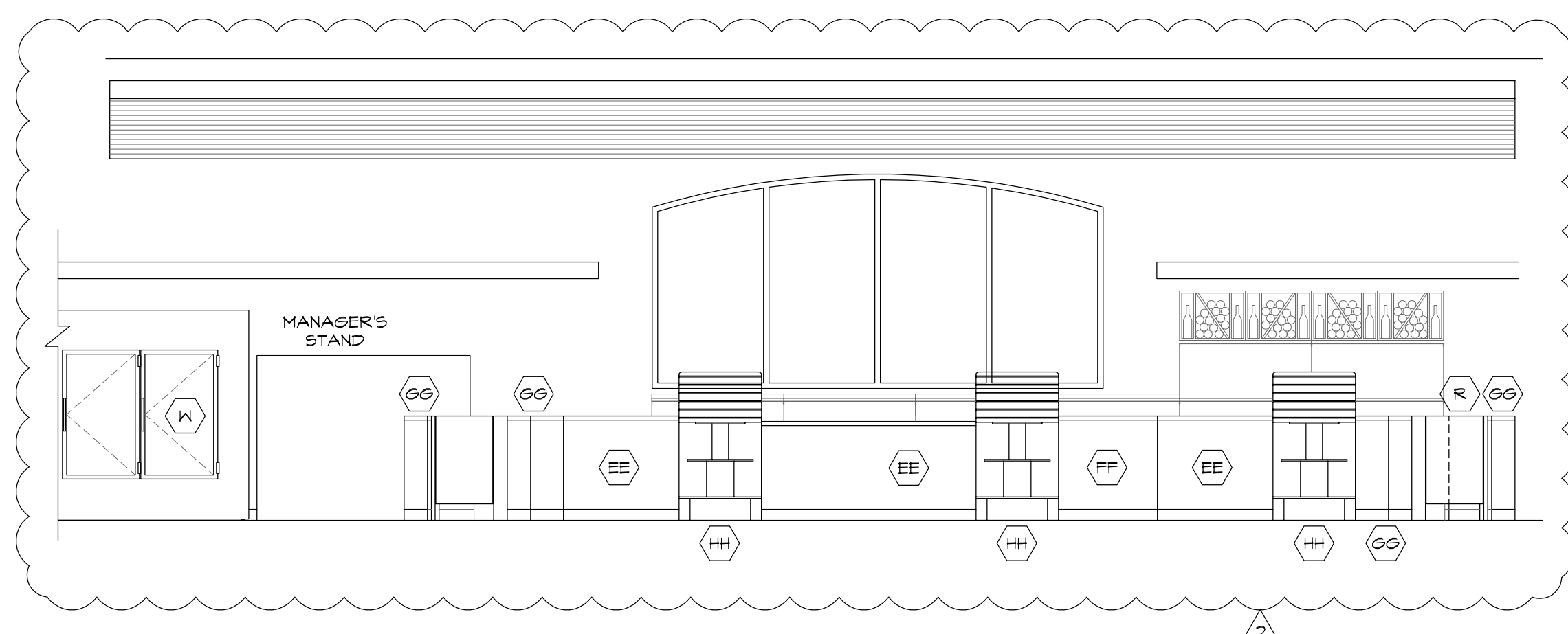
2 P.O.S. ELEVATION SCALE: 1/4" = 1'-0"
