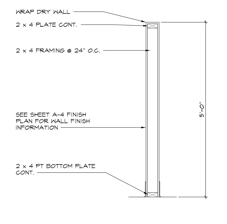
3 MANAGER STAND WALL DETAIL SCALE: 3/4" = 1'-0"
