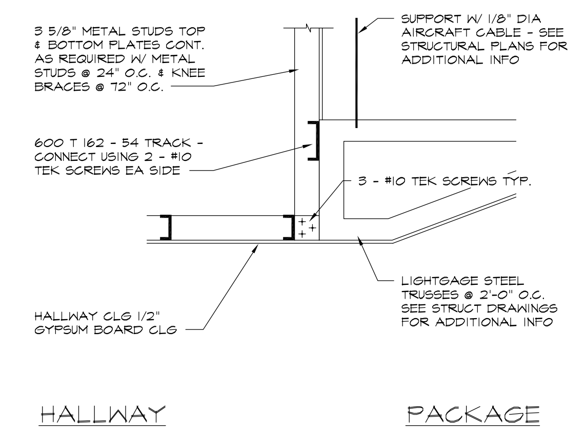
3 SECTION @ HALLWAY ENTRANCE SCALE: 3/4" = 1'-0"
