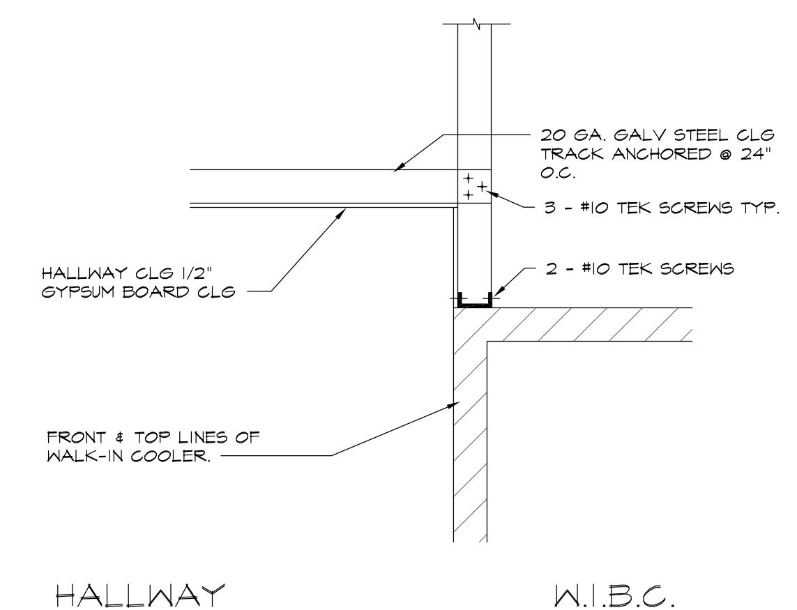
5 WALL ABOVE W.I.B.C. AT HALLWAY SCALE: 3/4" = 1'-0"
