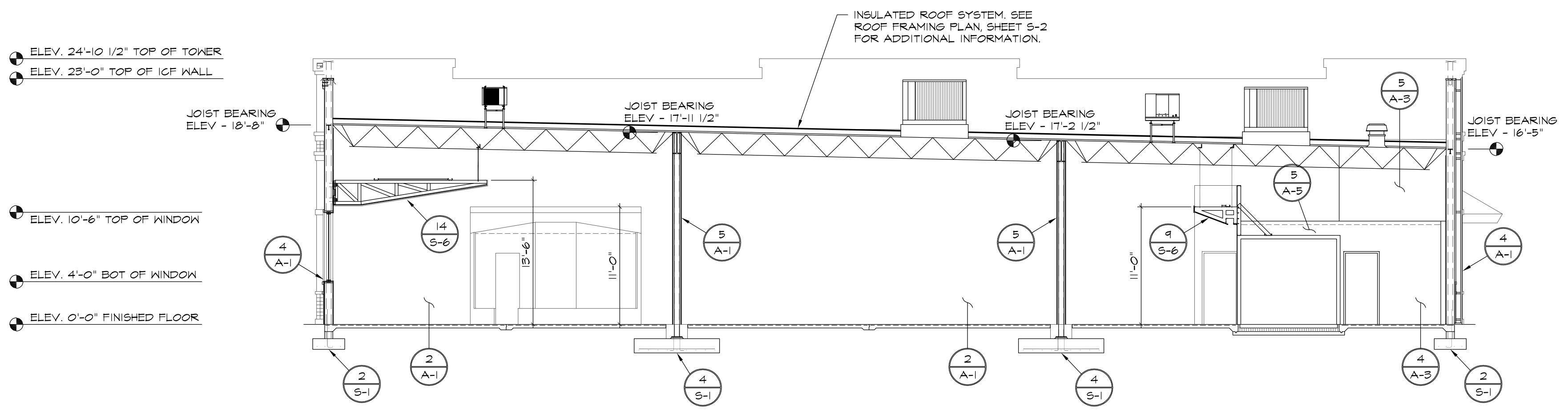
2 BUILDING SECTION SCALE: 1/8" = 1'-0"
