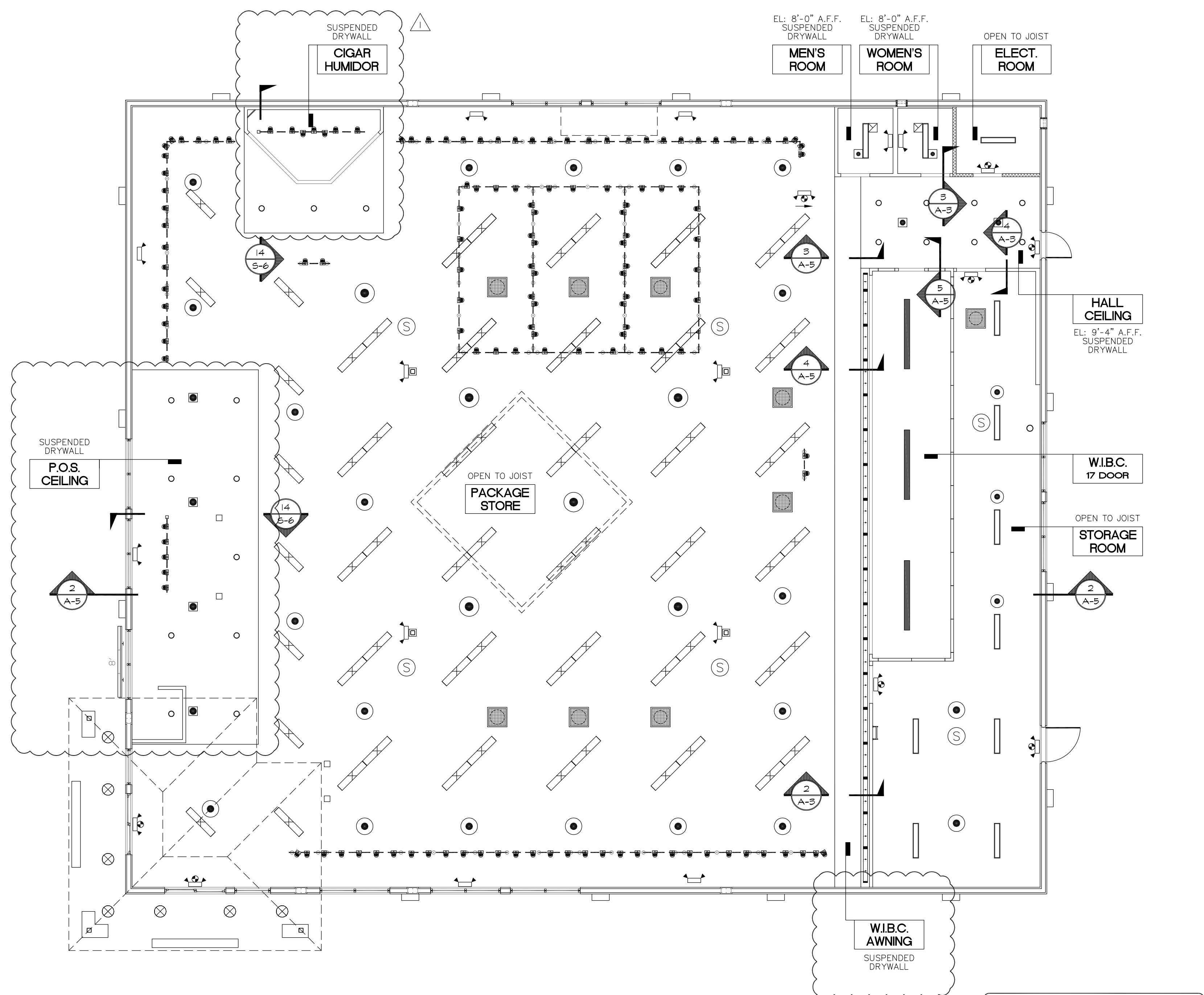
1 REFLECTED CEILING PLAN SCALE: 1/8" = 1'-0"
