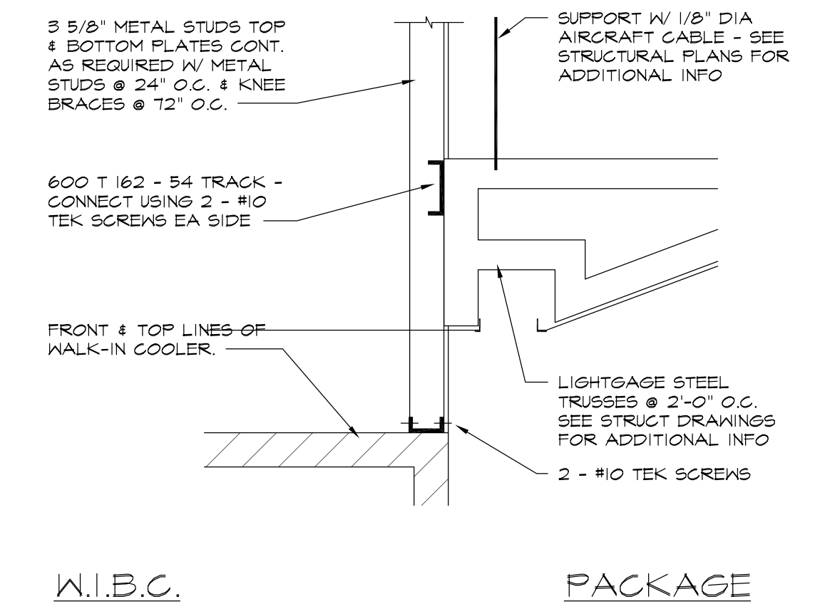
4 WALL ABOVE W.I.B.C. AT PACKAGE SCALE: 3/4" = 1'-0"
