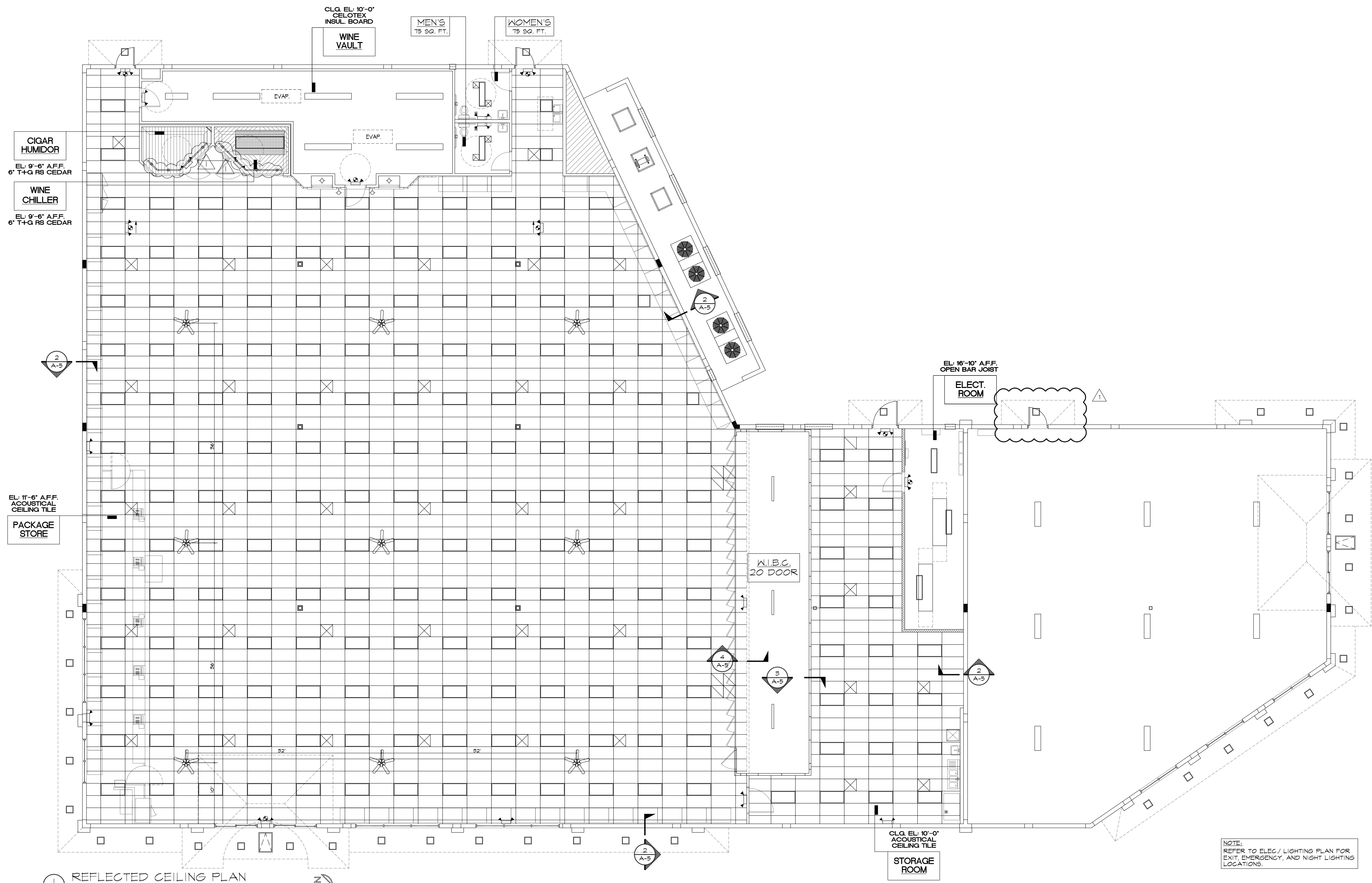
1 REFLECTED CEILING PLAN SCALE: 1/8" = 1'-0"
