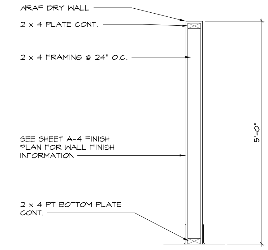
3 MANAGER STAND WALL DETAIL SCALE: 3/4" = 1'-0"
