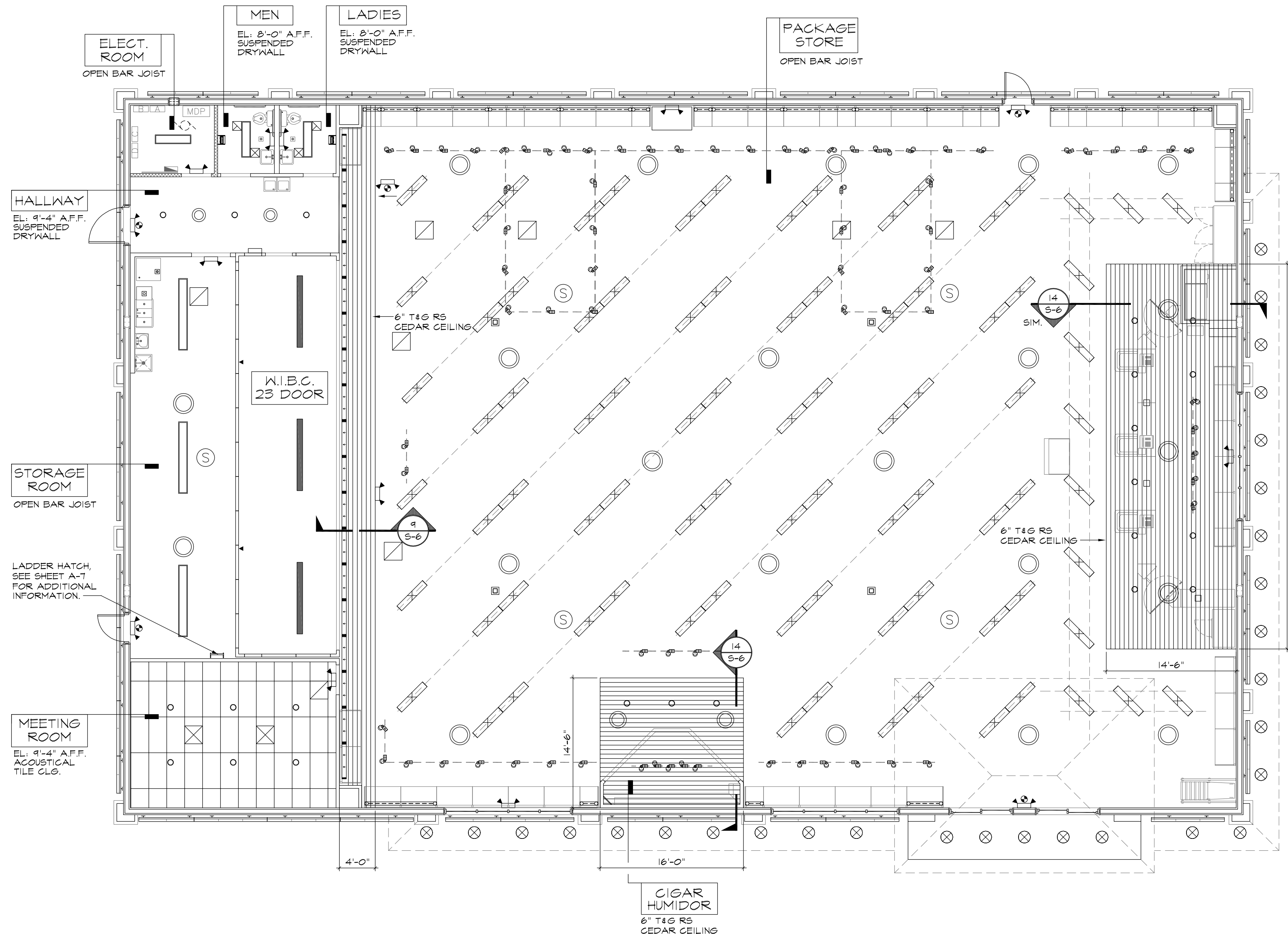
1 REFLECTED CEILING PLAN A-4 SCALE: 1/8" = 1'-0" TRUE PROJECT
