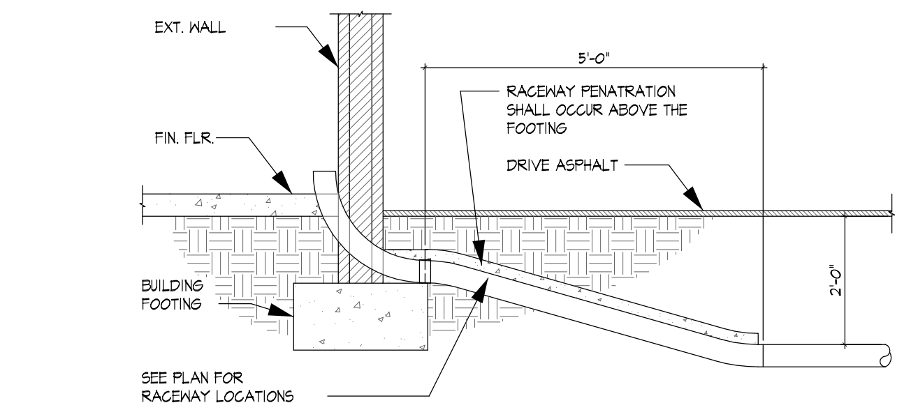
2 RACEWAY PENETRATION @ BUILDING SECTION E-3 NO SCALE
