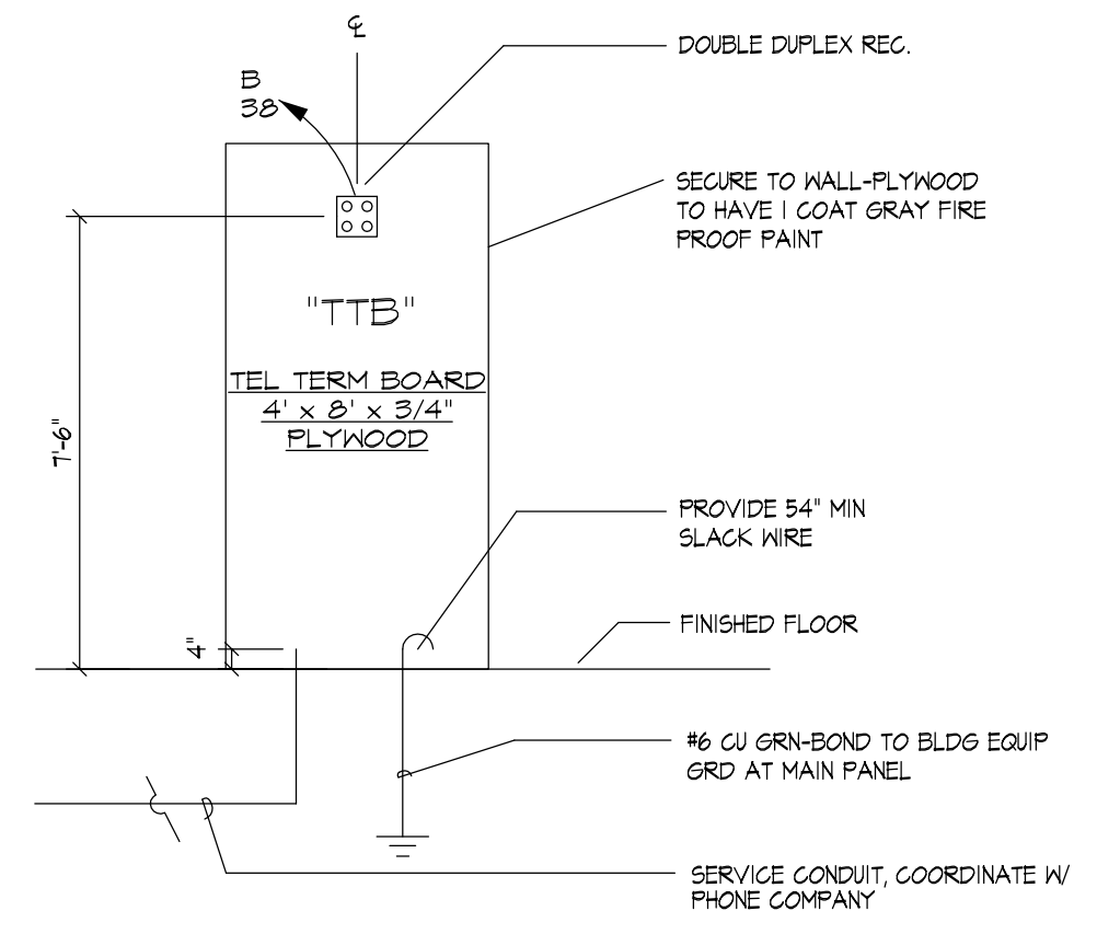
3 DETAIL 'A' E-3 NO SCALE
