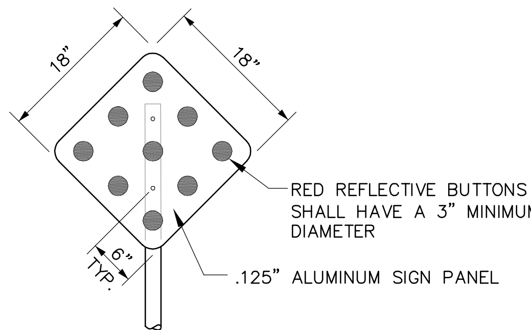
RED REFLECTIVE BUTTON SIGN N.T.S. FDOT INDEX NO. 17349
