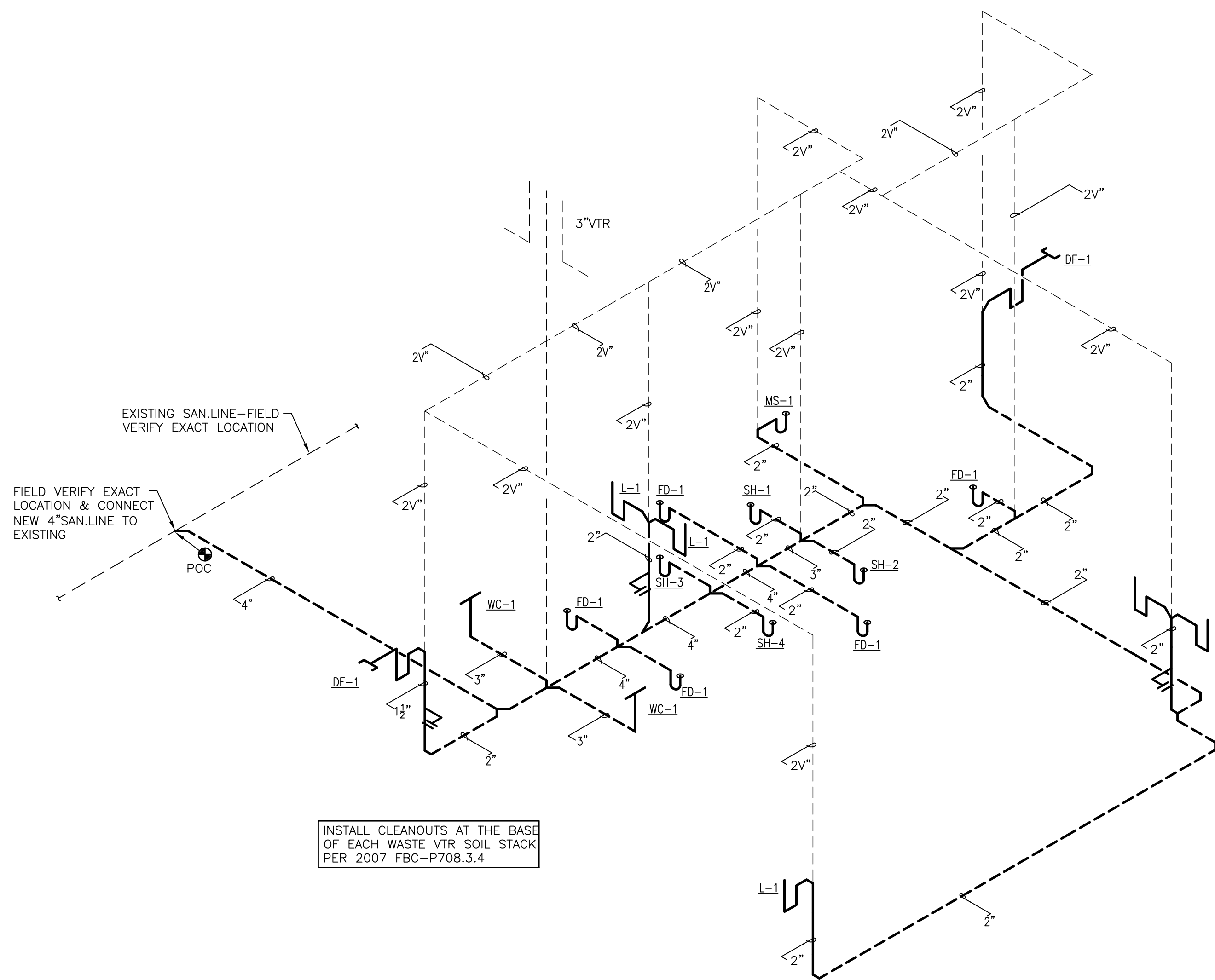
SANITARY RISER DIAGRAM
