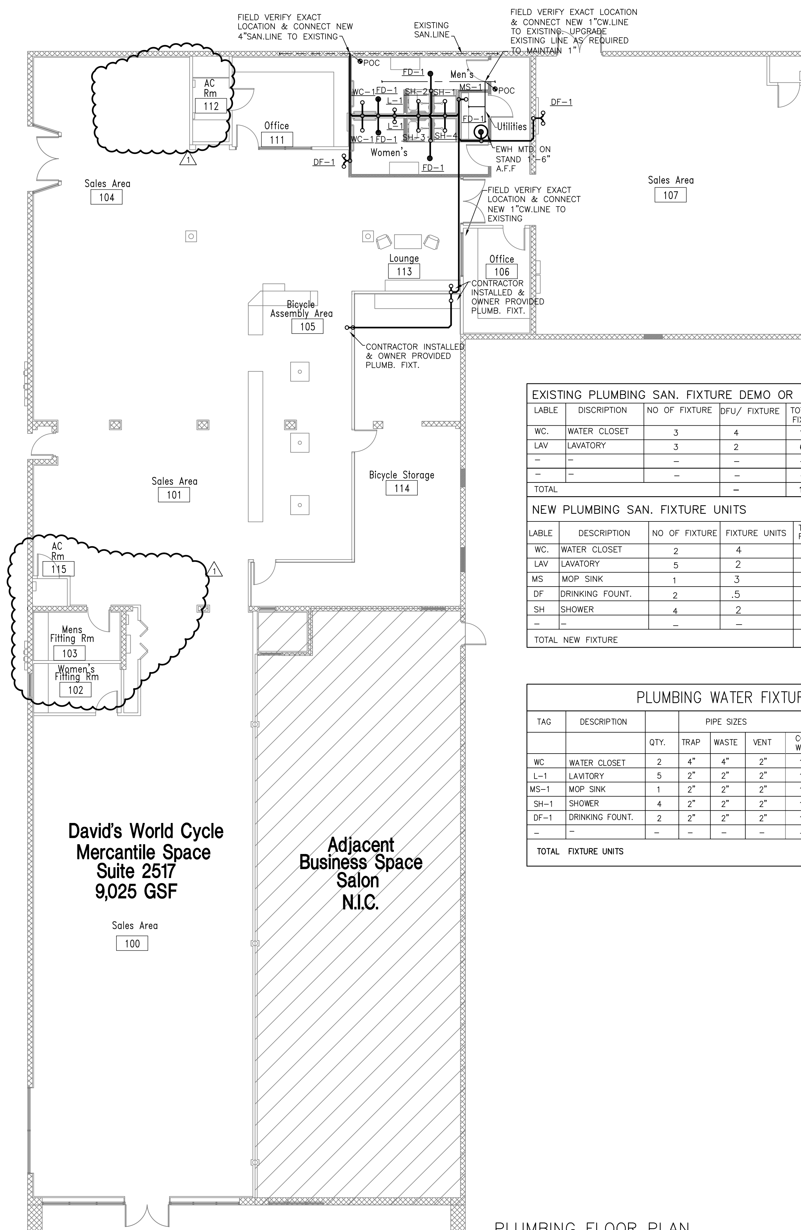
PLUMBING FLOOR PLAN
