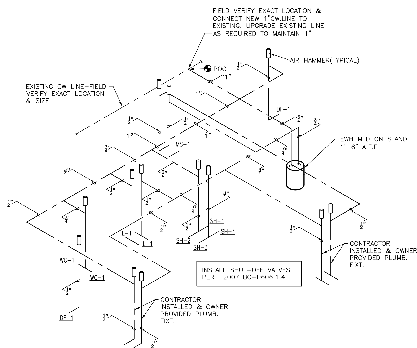
DOMESTIC WATER RISER DIAGRAM
