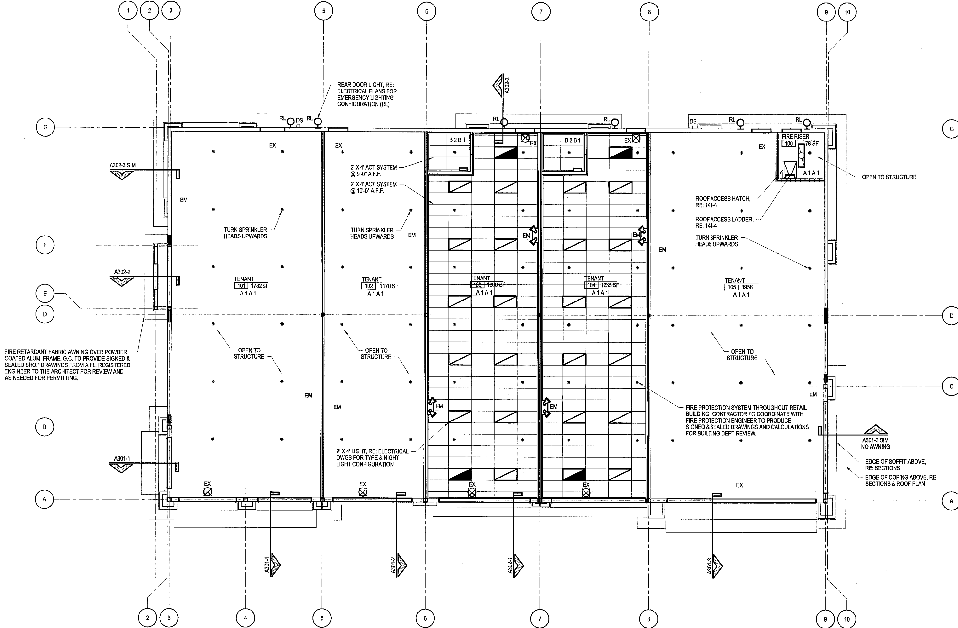
1 Reflected Ceiling Plan Scale: 1/8"=1'-0"
