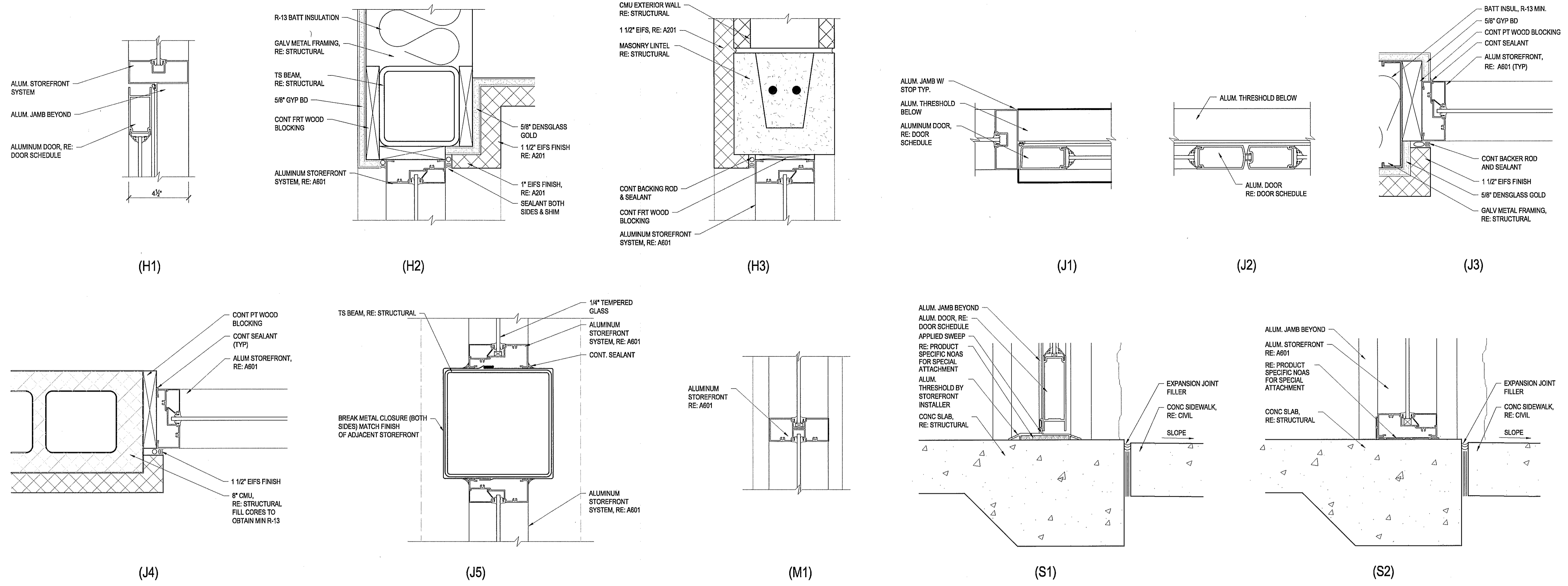
1 Storefront Head / Jamb / Sill Details Scale 3"=1'-0"
