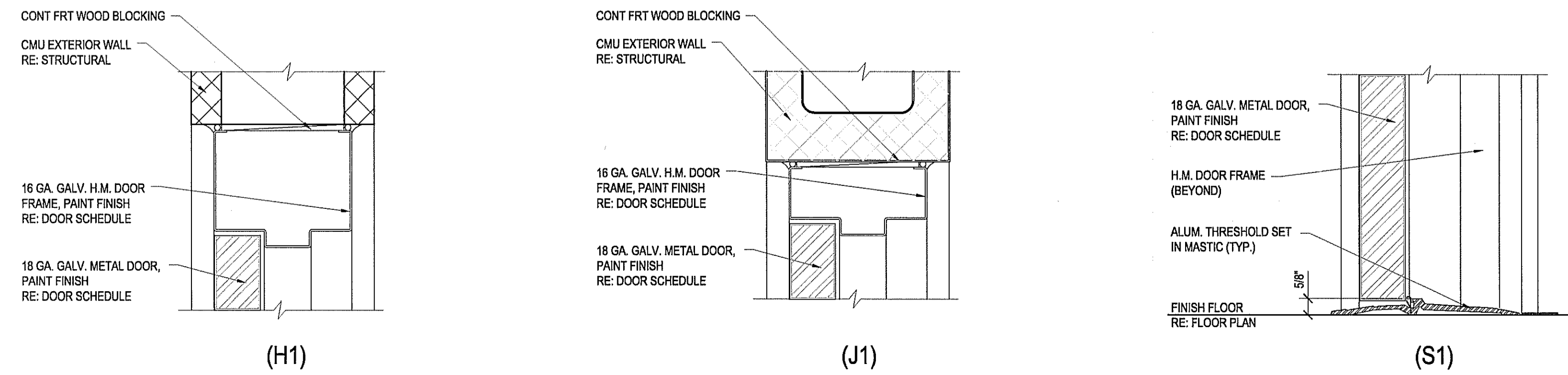
3 Hollow Metal Door Head / Jamb / Sill Details Scale 3"=1'-0"
