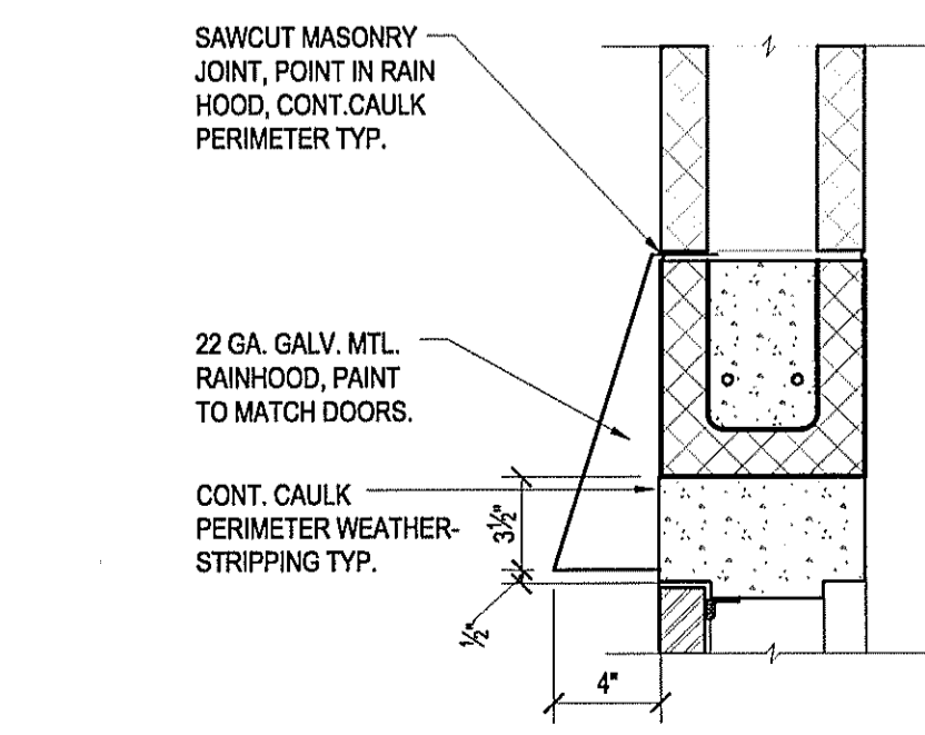
4 Rainhood Detail Scale 1 1/2"=1'-0"
