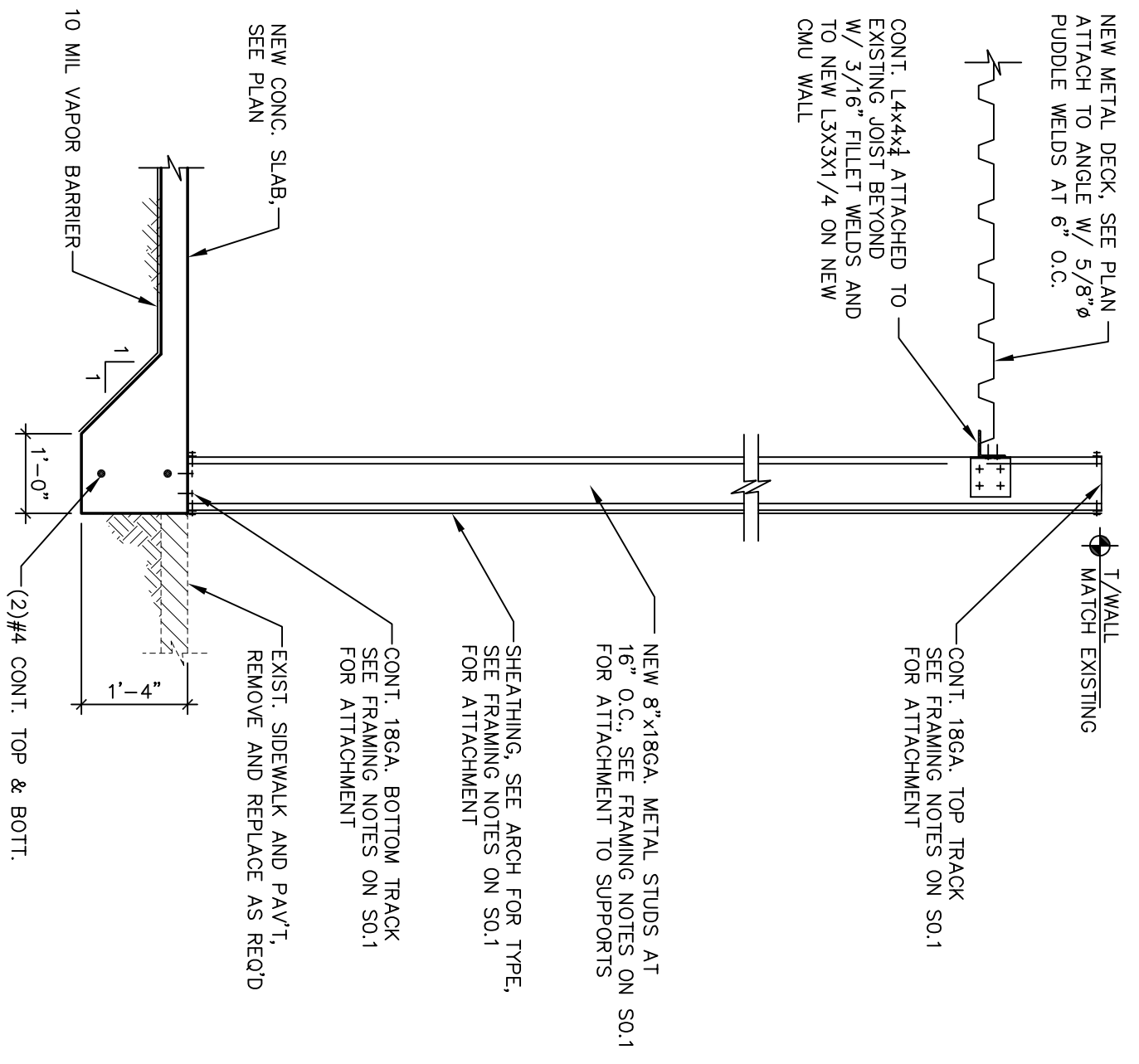
SECTION 3 S4.3 1/2" = 1'-0"
