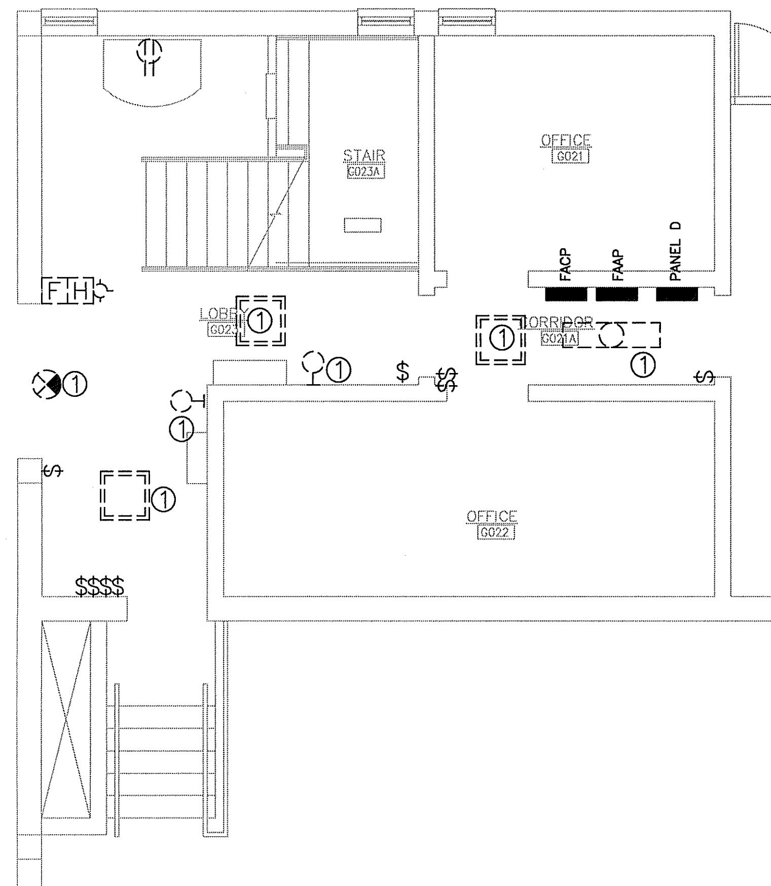
ELECTRICAL DEMOLITION PLAN - AREA A SCALE: 1/4"=1'-0"
