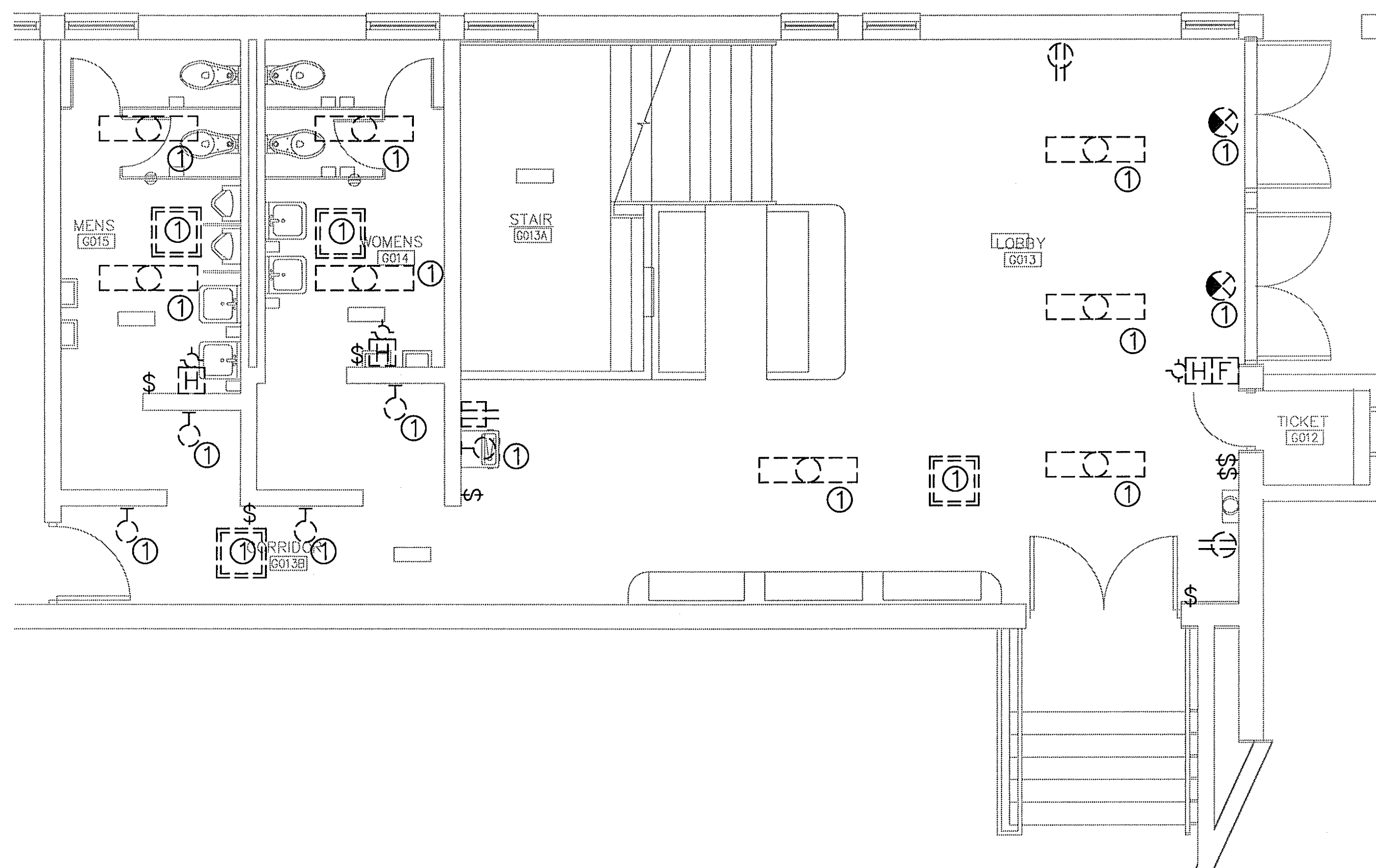
ELECTRICAL DEMOLITION PLAN - AREA B SCALE: 1/4"=1'-0"
