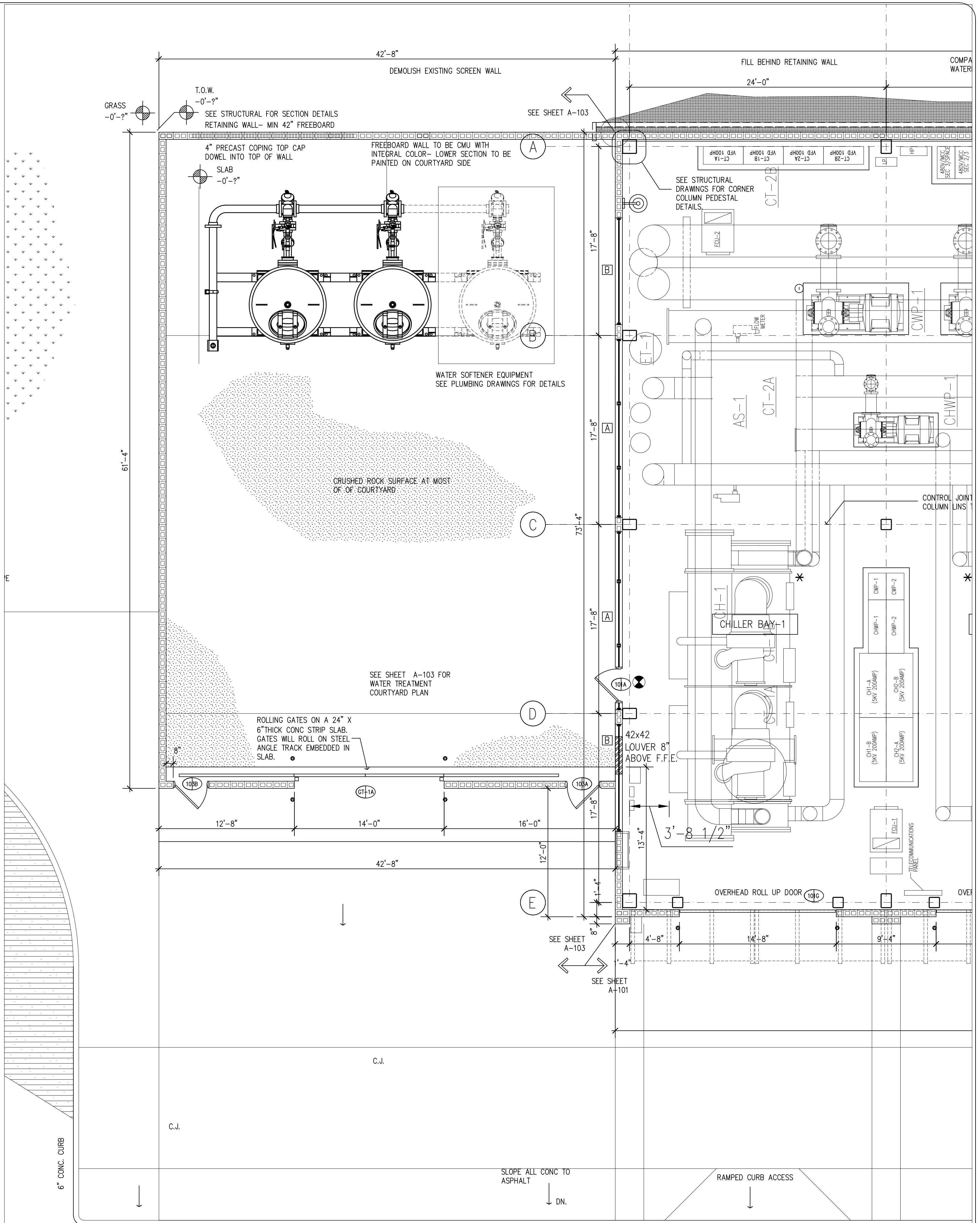
4 WATER TREATMENT COURTYARD PLAN SCALE: 3/16"=1'-0"
