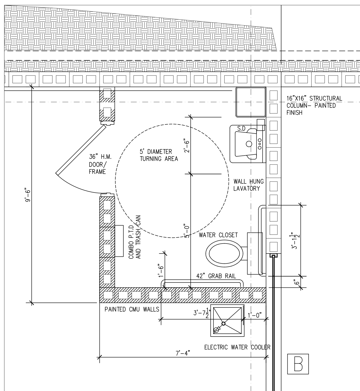
2 ENLARGED RESTROOM PLAN SCALE: 1/2"=1'-0"
