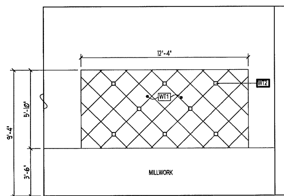
TILE FLOOR PATTERN
