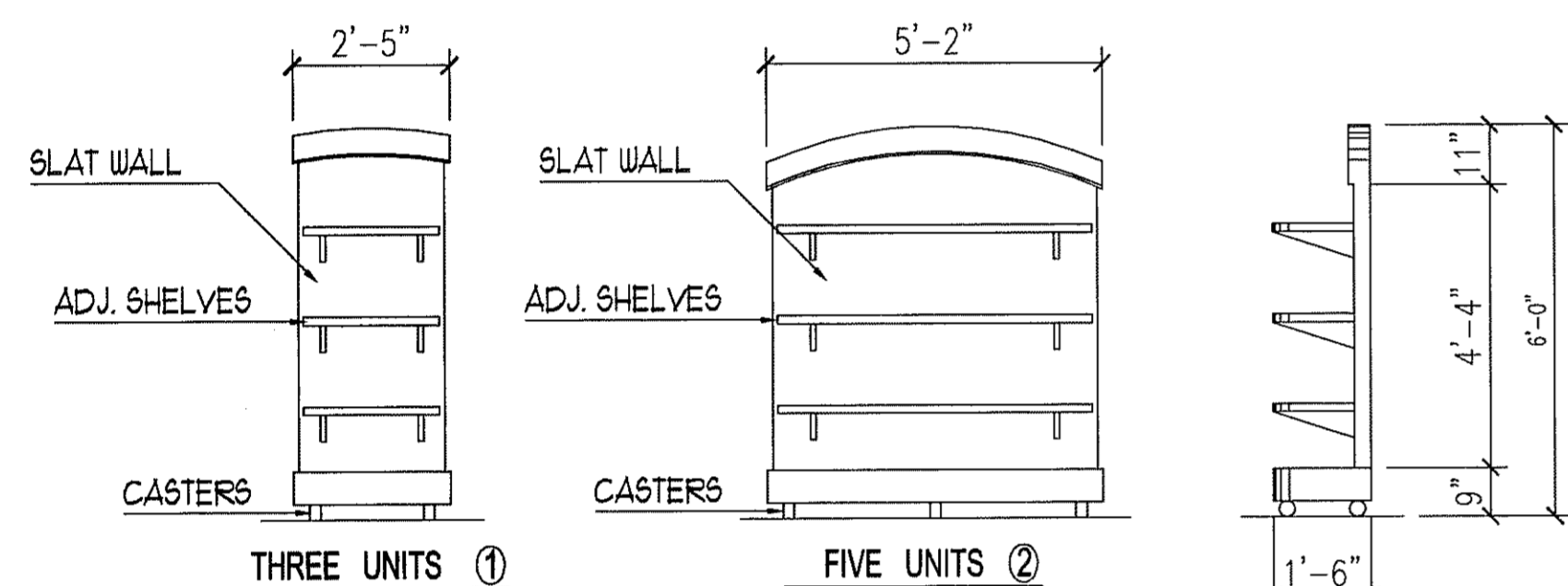
DISPLAY / STORAGE UNIT ELEVATIONS
