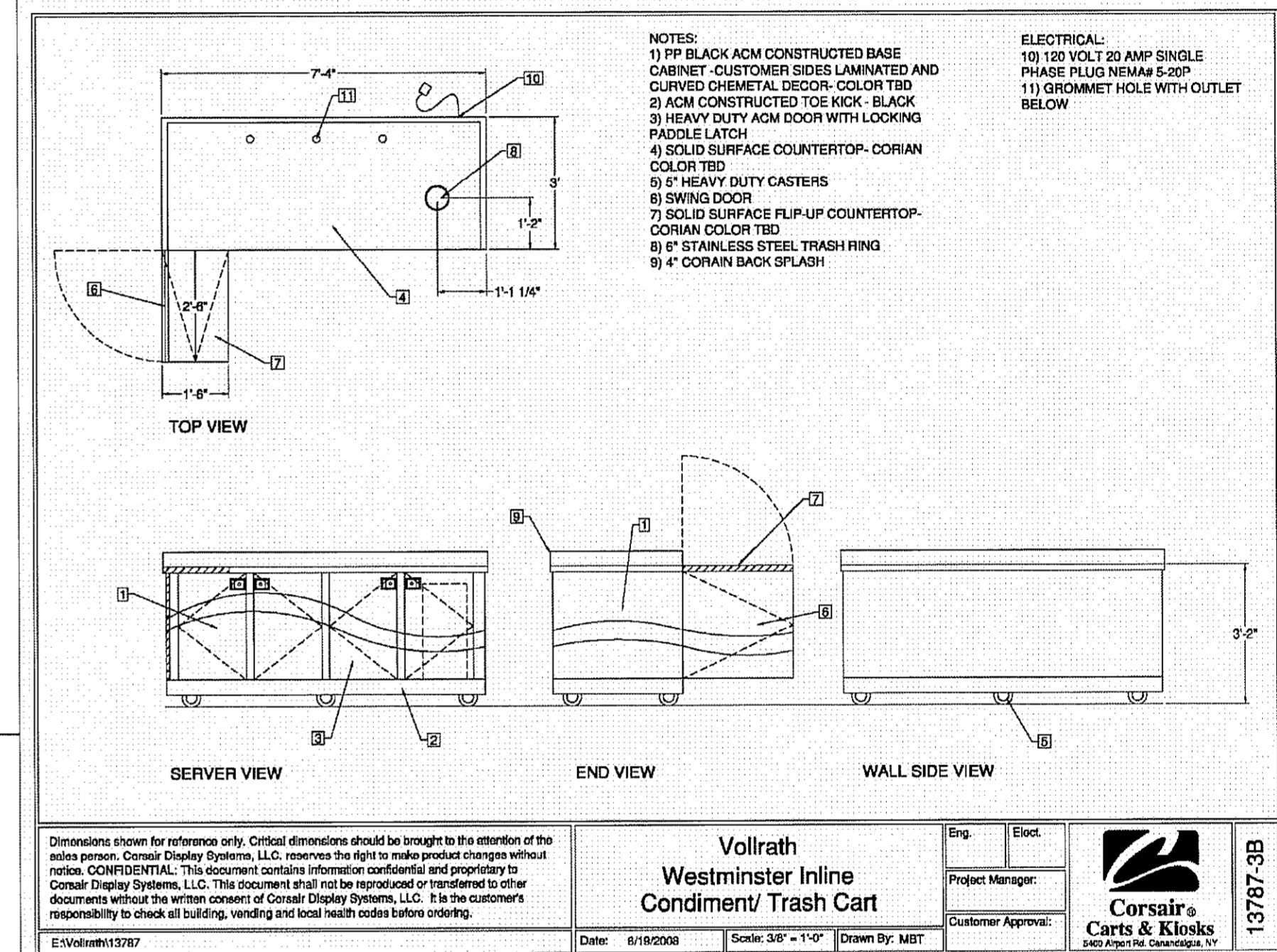
Vollrath Westminster Inline Back Cart Date: 6/18/2008 Scale: 1/4" = 1'-0" Drawn By: MBT Corsair & Kloske 13787-2B
