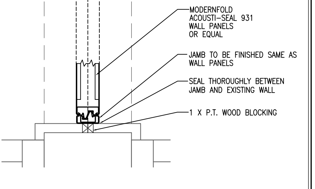
11 WALL PANEL JAMB DETAIL IA601 SCALE: 1 1/2" = 1'-0"
